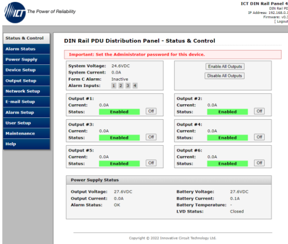
Figure 4. GUI with Power Supply and Battery status
